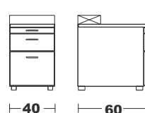
Upper support pedestal
